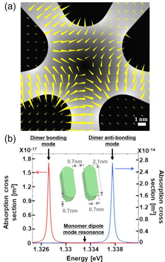
図 1 (a) Optical nanovortex formed when the resonant localized surface plasmon of the nanogap of a gold pentamer nanostructure is excited by a Laguerre-Gaussian laser beam ( \ell=1 ). (b) Absorption cross-sections of a model dimer molecule placed in the nanogap of a gold pentamer nanostructure under (red curve) Gaussian beam and (blue curve) Laguerre-Gaussian laser beam ( \ell=1 ) irradiation.
