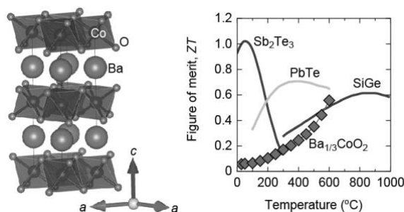
FIG. 1 | (Left) Schematic crystal structure of \text{Ba}_{1/3}\text{CoO}_2 . (Right) Temperature dependence of the ZT of the \text{Ba}_{1/3}\text{CoO}_2 epitaxial film in the in-plane direction. Comparison against commercially available p-type thermoelectric materials. The ZT of the \text{Ba}_{1/3}\text{CoO}_2 epitaxial film at 600 °C is comparable to that of p-type PbTe and p-type SiGe.
